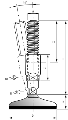
Dimensioned Drawing Sunnex H3A-Series
