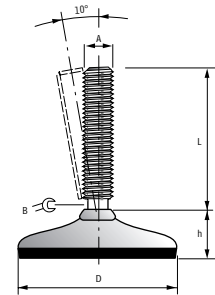
Dimensioned Drawing Sunnex H
