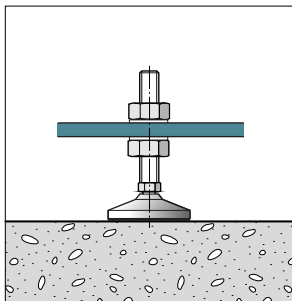
Assembly example Sunnex LL-Series
