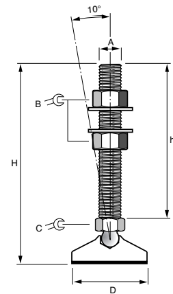
Dimensioned Drawing Sunnex LL-Series
