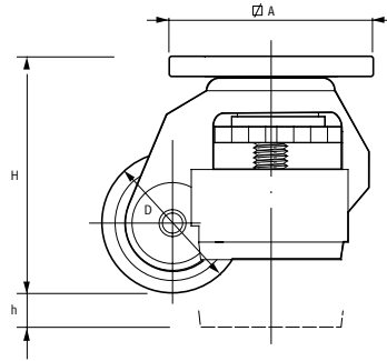
Dimensioned Drawing SLC Type A: Plate Mounting
