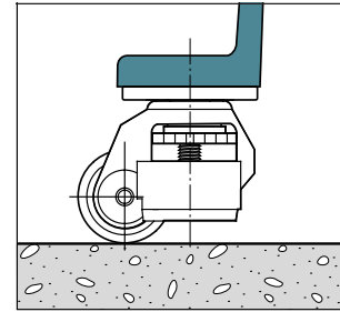
Assembly example SLC Type A: Plate Mounting
