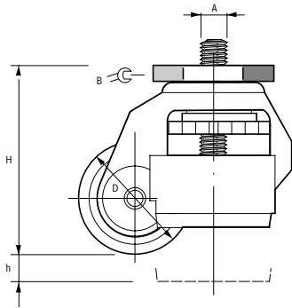
Dimensioned Drawing SLC Type A: Stud Mounting
