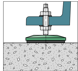
Assembly example Sunnex SM-Series
