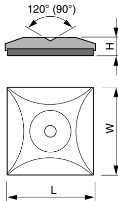
Dimensioned Drawing Sunnex SM-Series
