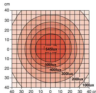
CL Series Lux Table 9W
