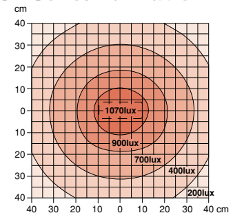
CL Series Lux Table 11W
